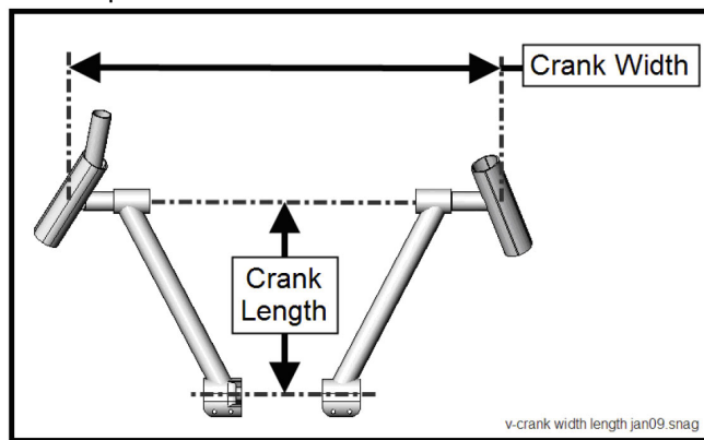
Optional V-Crankset Measurement Guideline
